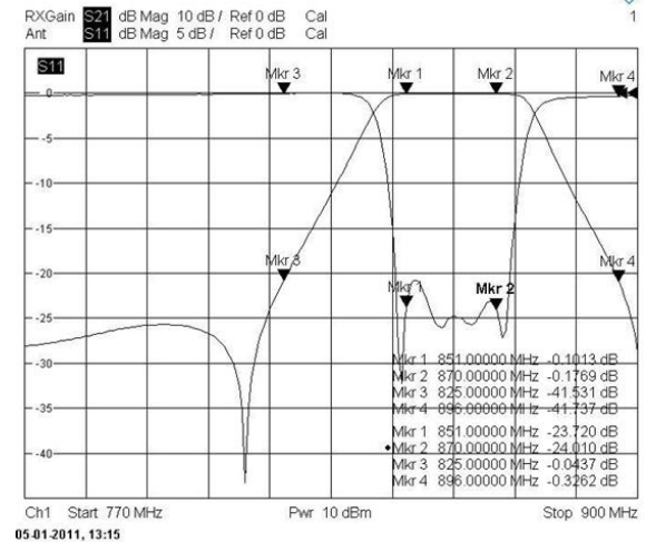
Typical filter mask, 800 MHz
